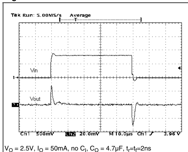
Figure 13. Line transient
