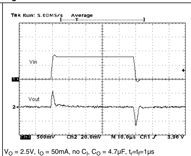
Figure 14. Line transient
