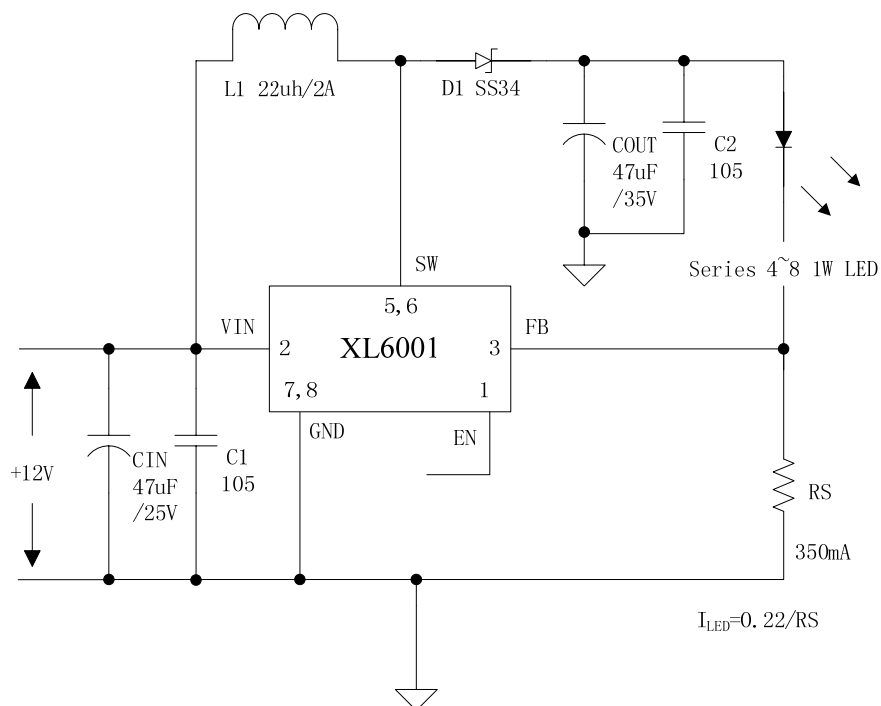
Figure4. XL6001 Typical Application Circuit
