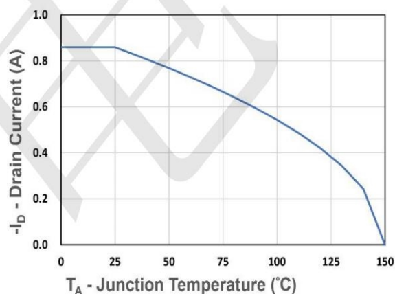
Figure 10. Drain Current
