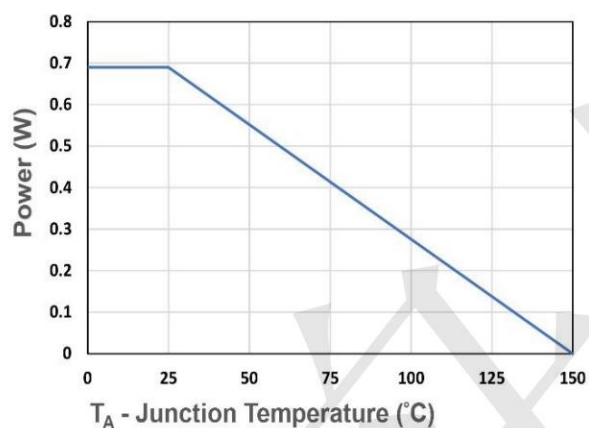
Figure 9. Power Dissipation
