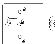
Wiring Diagram (Bottom View)
