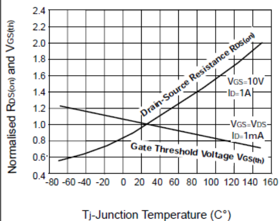
Normalised R_{DS(on)} and V_{GS(th)} v Temperature
