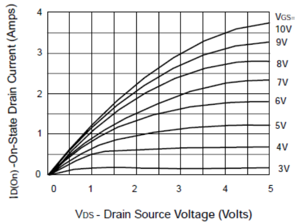
Saturation Characteristics
