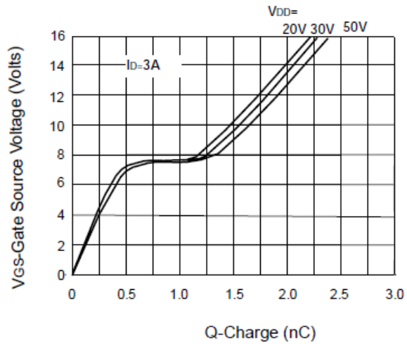
Gate charge v gate-source voltage
