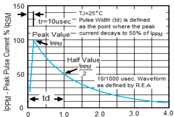
Fig.3 Pulse Waveform
