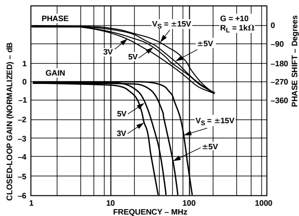
Figure 32. Closed-Loop Gain and Phase vs. Frequency, Gain = +10, R_L = 1 k\Omega
