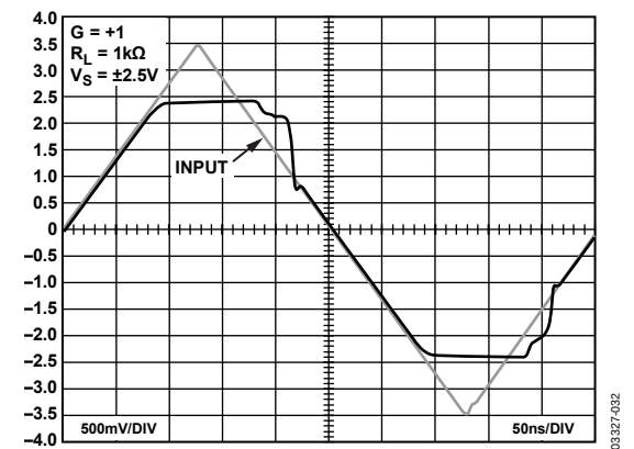
Figure 37. Overdrive Recovery, G = +1
