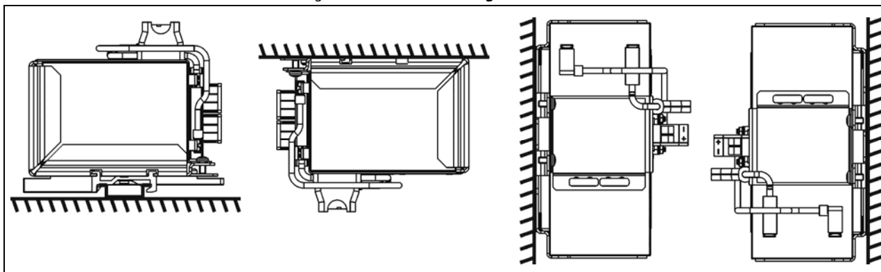
Fig. 19-2 Allowed mounting orientations
