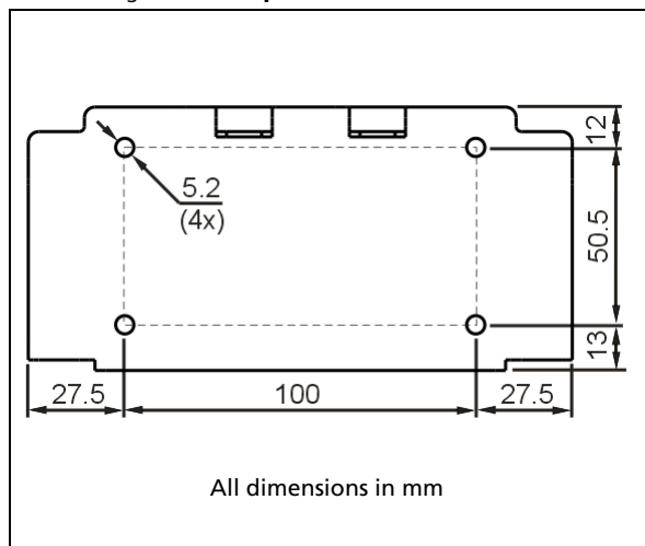
Fig. 17-3 Hole pattern for bottom mount
