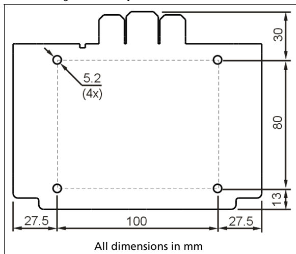
Fig. 17-2 Hole pattern for wall mount
