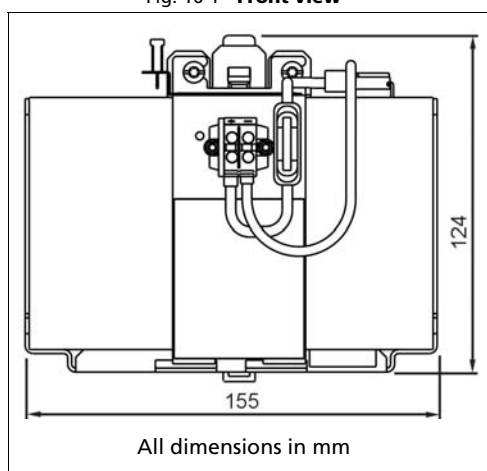
Fig. 16-1 Front view
