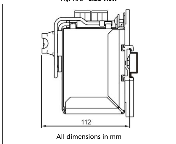
Fig. 16-2 Side view
