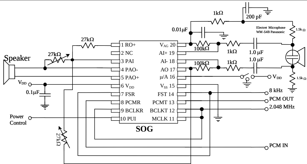
Figure 11.3 Handset Interface
