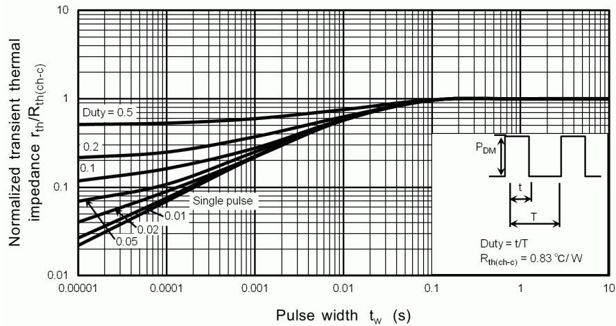
Fig. 8.18 r_{th}/R_{th(ch-c)} - t_w (Guaranteed Maximum)
