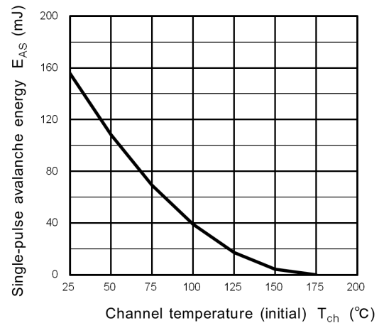
Fig. 8.16 E_{AS} - T_{ch} (Guaranteed Maximum)
