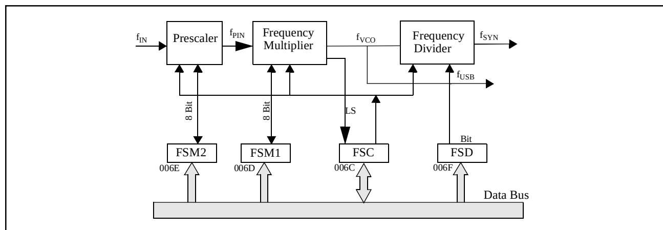
Fig. 1.91. Frequency Synthesizer Circuit
