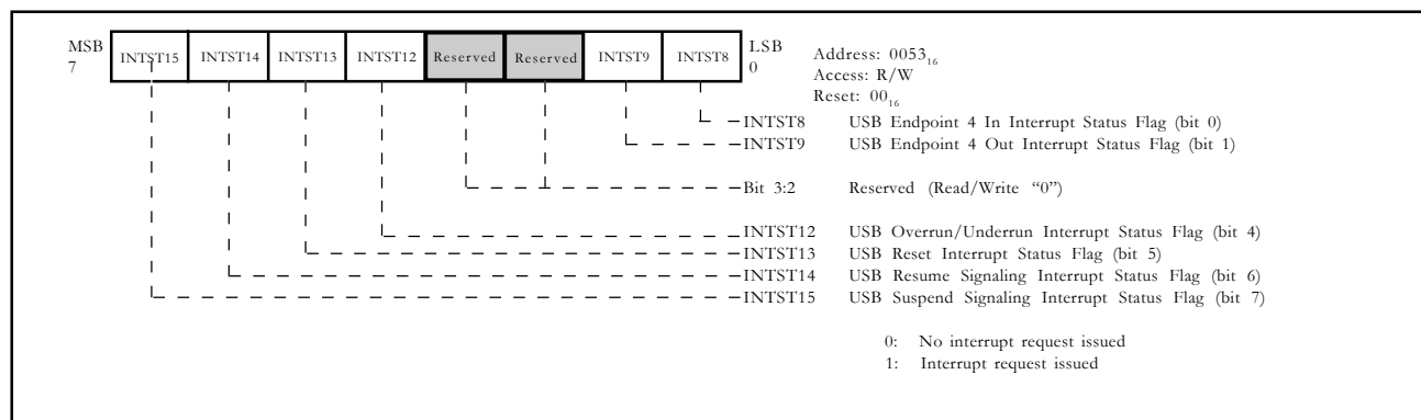
Fig. 1.56. USB Interrupt Status Register 2 (USBIS2)
