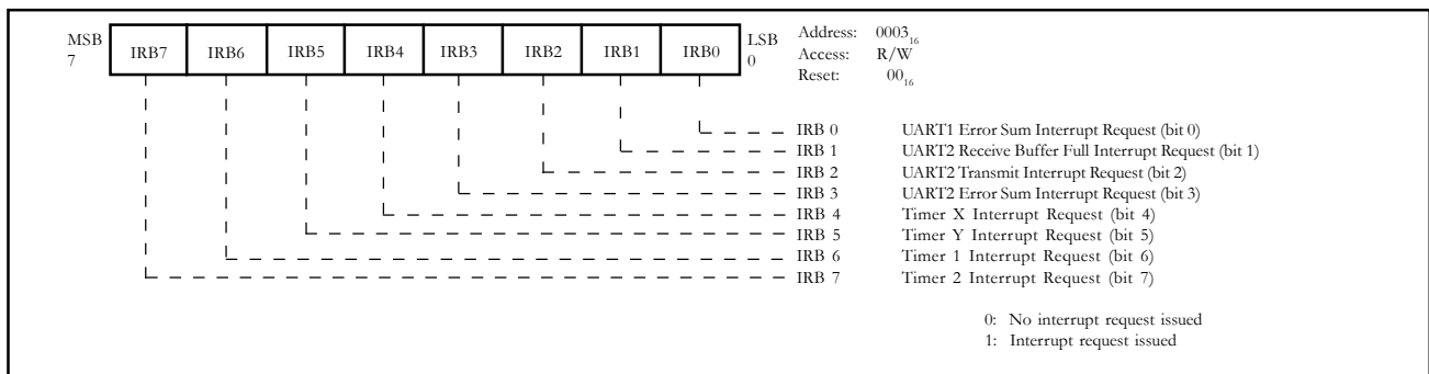
Fig. 1.25. Interrupt Request Register B (IREQB)
