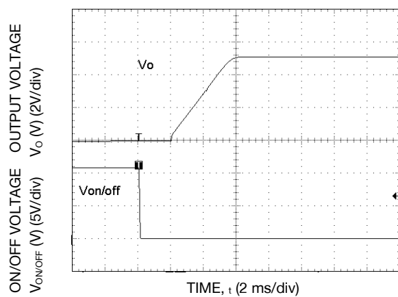
Start-up Using On/Off Voltage ( I_o = I_{o, max} ), V_o = 5.0V
