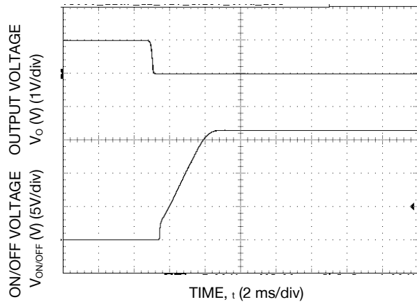
Start-up Using On/Off Voltage ( I_o = I_{o, max} ), V_o = 3.3V
