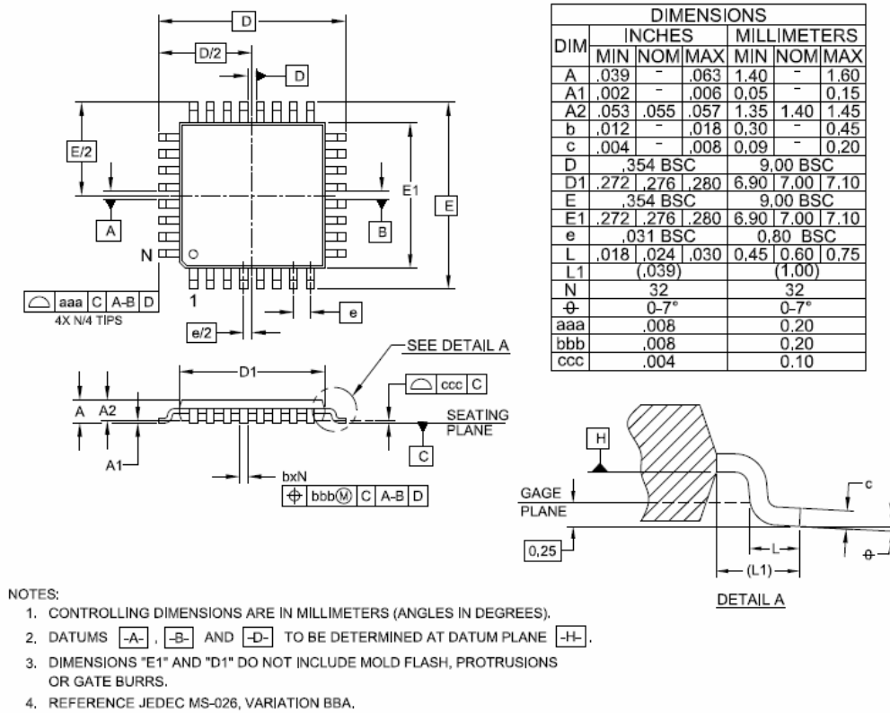
Figure 63 Package Outline Drawing
