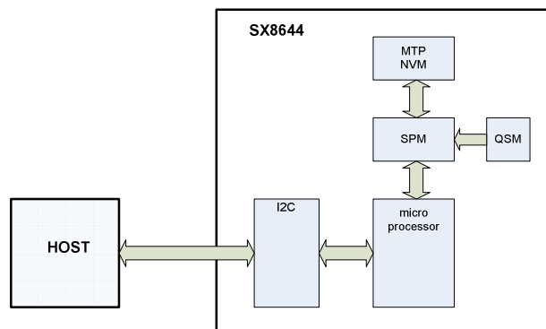
Figure 20 Configuration
