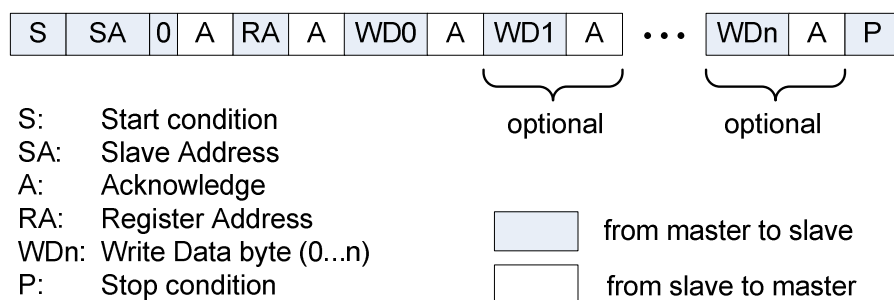
Figure 54 I2C write
