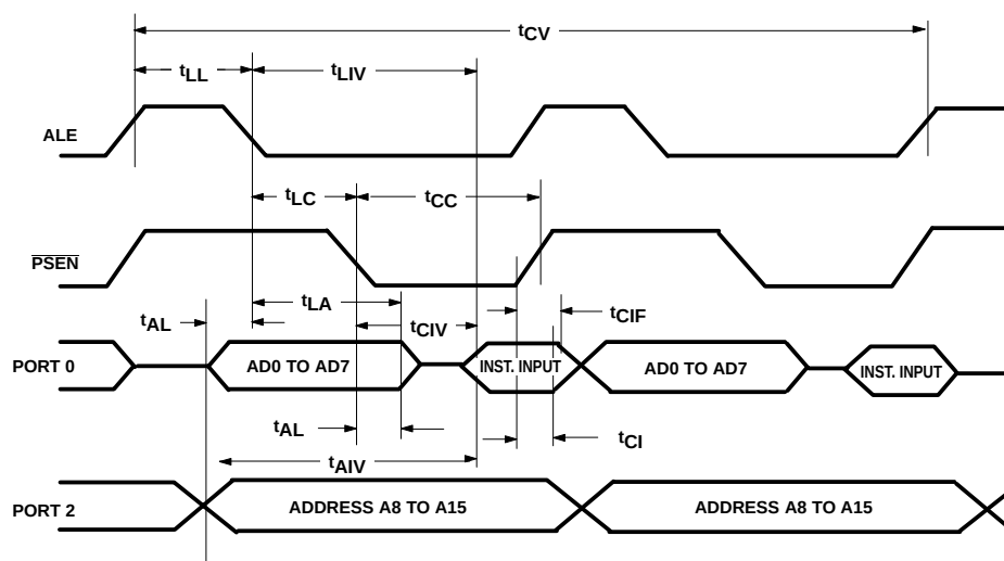
Figure 20. Read from Program Memory
