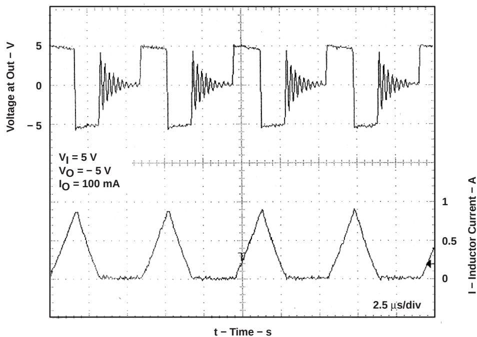
Figure 2. Switching Waveforms
