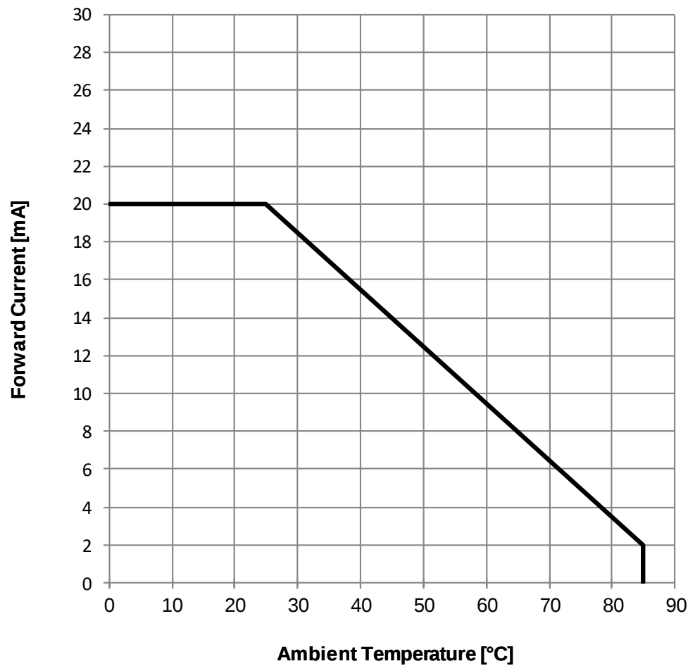
Derating Curve:
