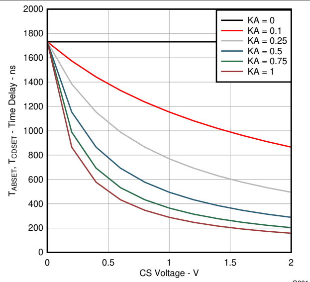
图 7-3. Delay Time set T_{ABSET} and T_{CDSET} (Over CS Voltage Variation and Selected K_A for R_{AB} and R_{CD} Equal 90 k \Omega )
