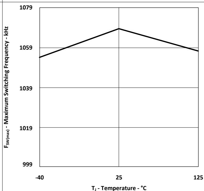
图 6-12. Maximum Switching Frequency vs Temperature
