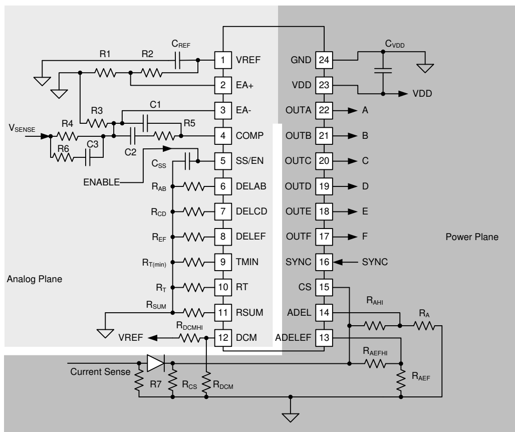
图 7-18. Layout Recommendation for Analog and Power Planes
