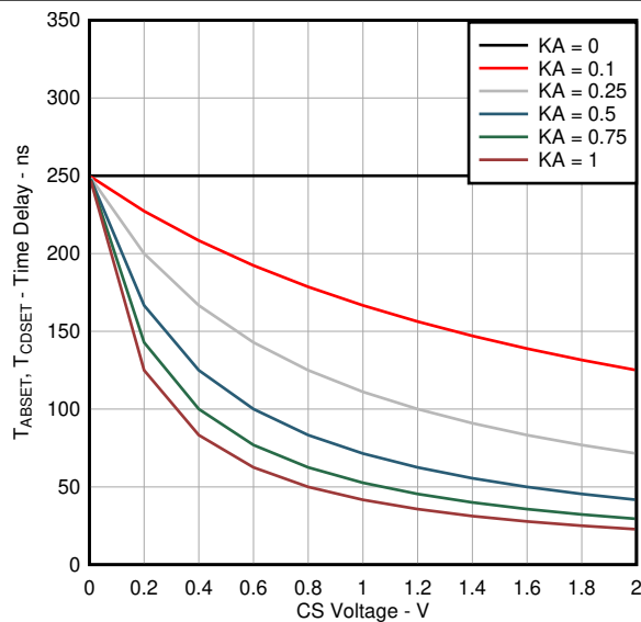
图 7-2. Delay Time Set T_{ABSET} and T_{CDSET} (Over CS Voltage Variation and selected K_A for R_{AB} and R_{CD} Equal 13 k \Omega )
