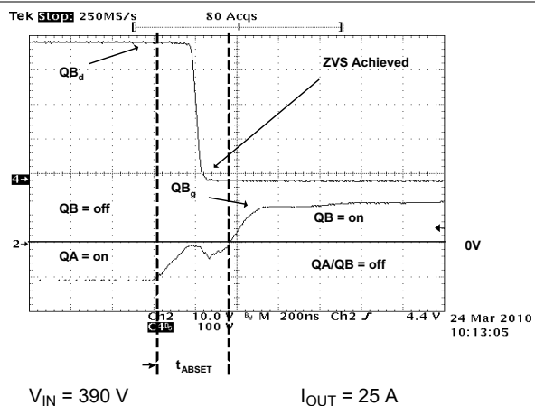
图 8-15. Full-Bridge Gate Drives and Switch Nodes (QB g QB d )
