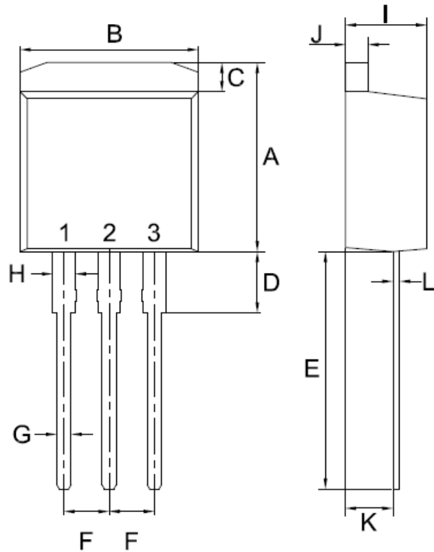
TO-262 (I² PAK)
