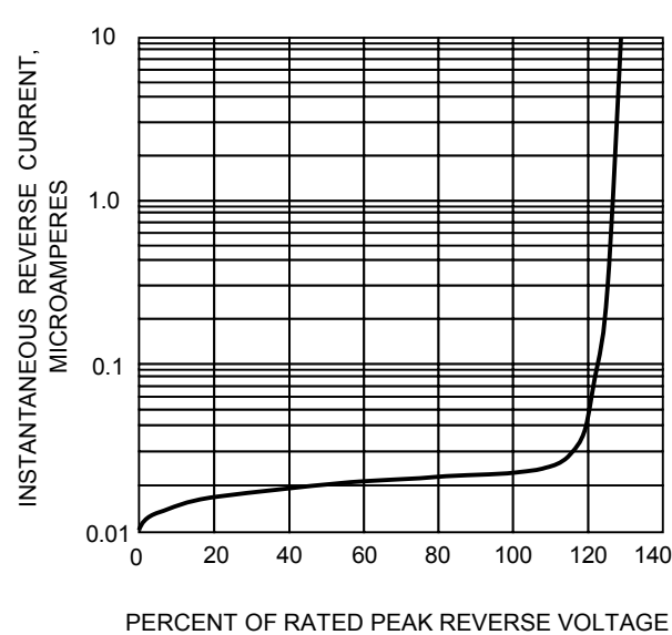
FIG.4-TYPICAL REVERSE CHARACTERISTICS
