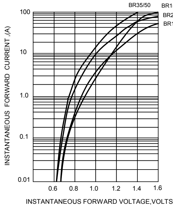
FIG.3-TYPICAL FORWARD CHARACTERISTICS
