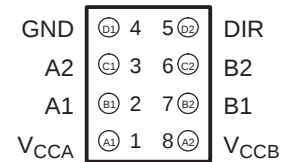
YZP PACKAGE (BOTTOM VIEW)
