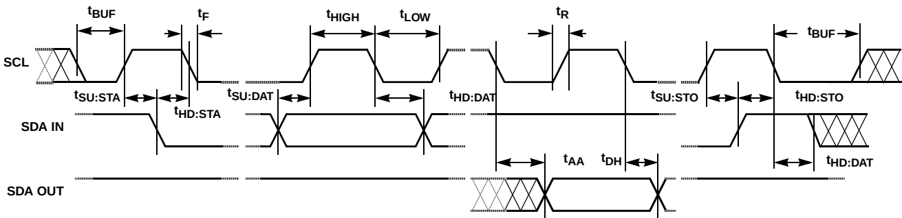
FIGURE 4. BUS TIMING
