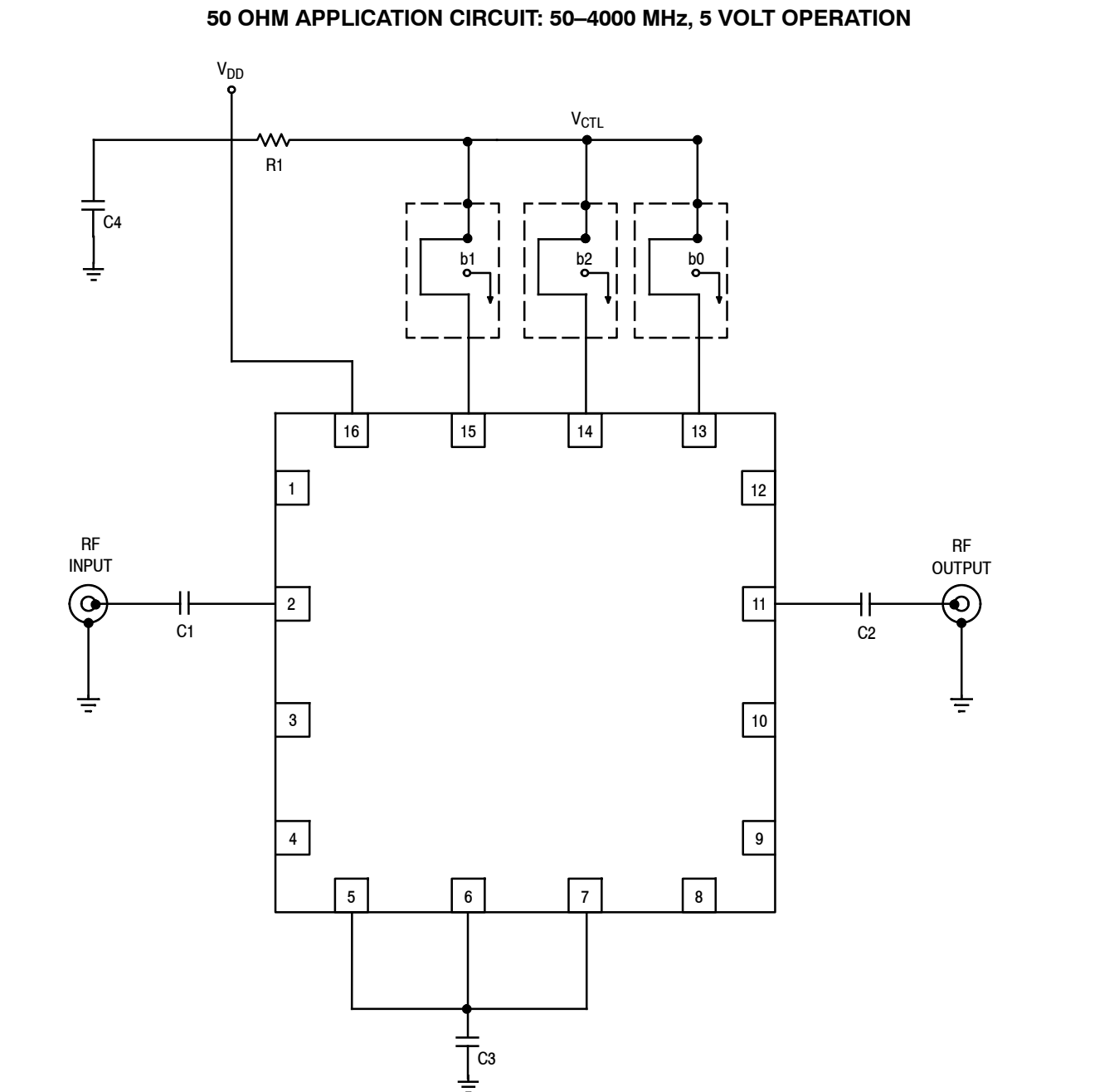
Figure 3. MMT20303HT1 Test Circuit Schematic
