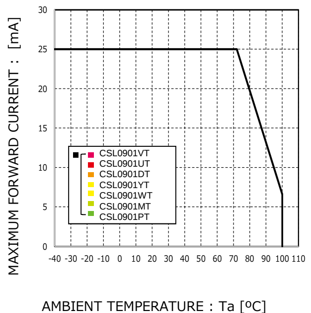
Fig.4 Derating
