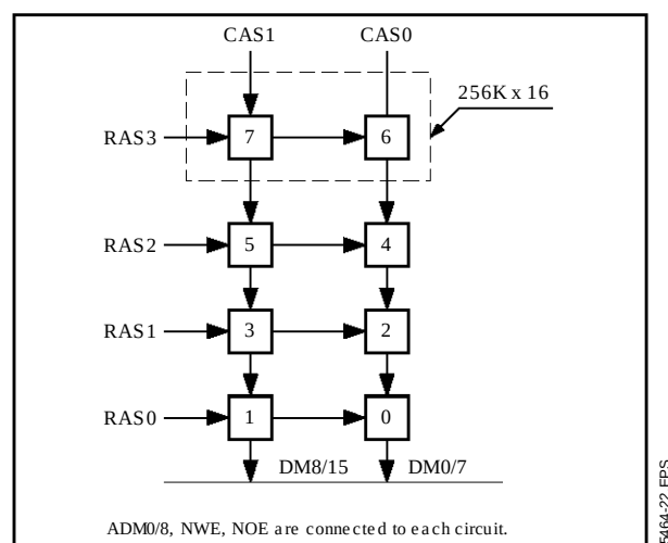
Figure 20 : 256K x 16 DRAM Circuit Organization
