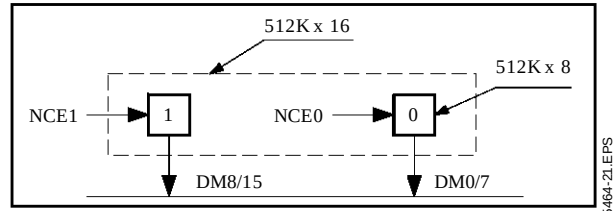
Figure 19 : 512K x 8 SRAM Circuit Memory Organization
