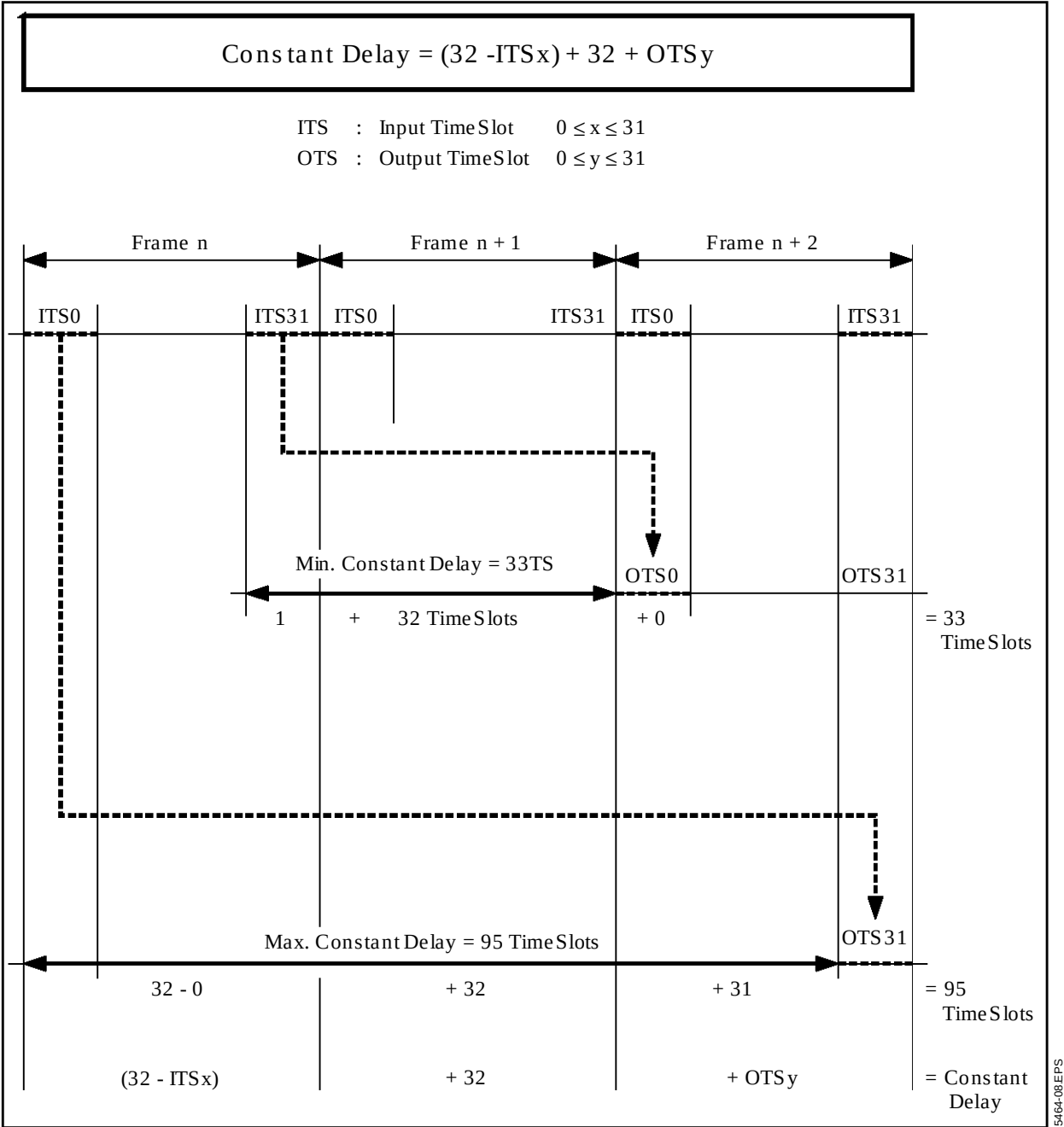
Figure 7 : Constant Delay through the matrix with SI = 1
