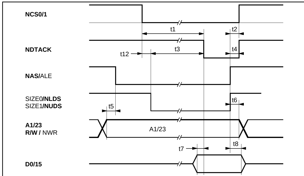
Figure 41 : 68000 Read Cycle
