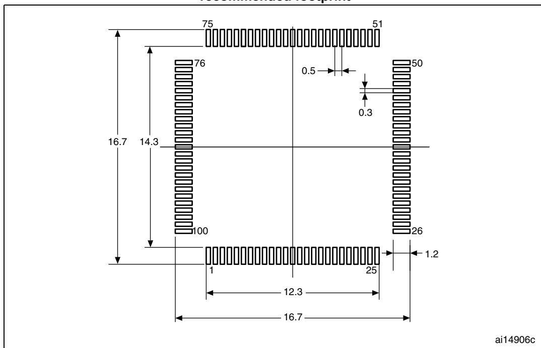
Figure 39. LQPF100 - 100-pin, 14 x 14 mm low-profile quad flat package recommended footprint
