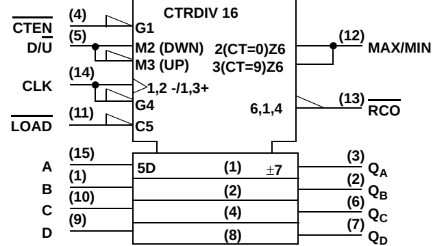
LOGIC SYMBOL
