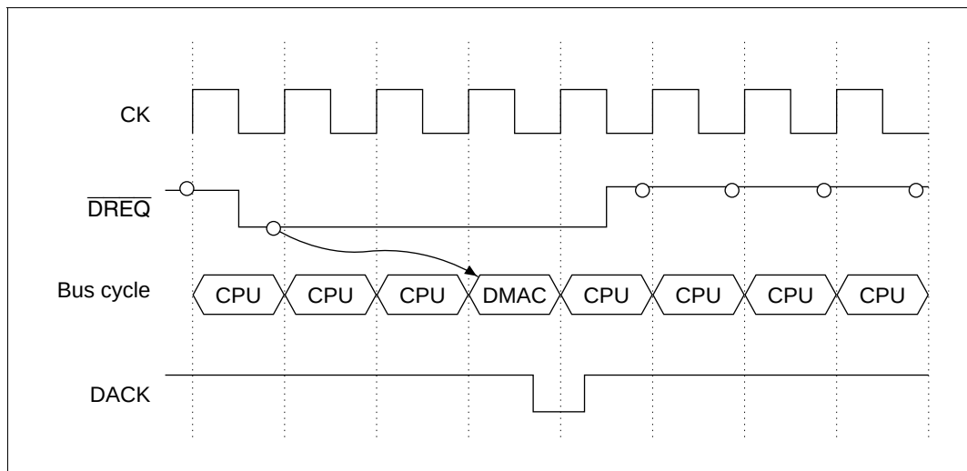
Figure 9.13 \overline{\text{DREQ}} Sampling Timing in Cycle Steal Mode (Output with \overline{\text{DREQ}} level detection and \overline{\text{DACK}} active low) (Single address mode, bus cycle = 1 state)
