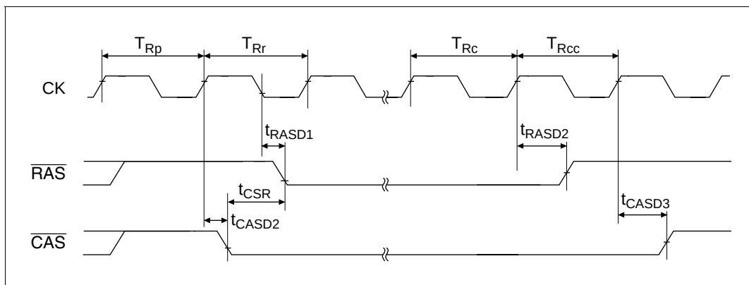
Figure 19.18 Self Refresh
