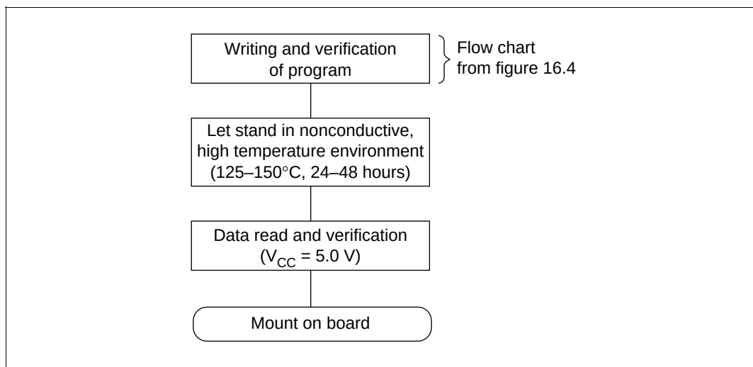
Figure 16.6 Screening Flow
