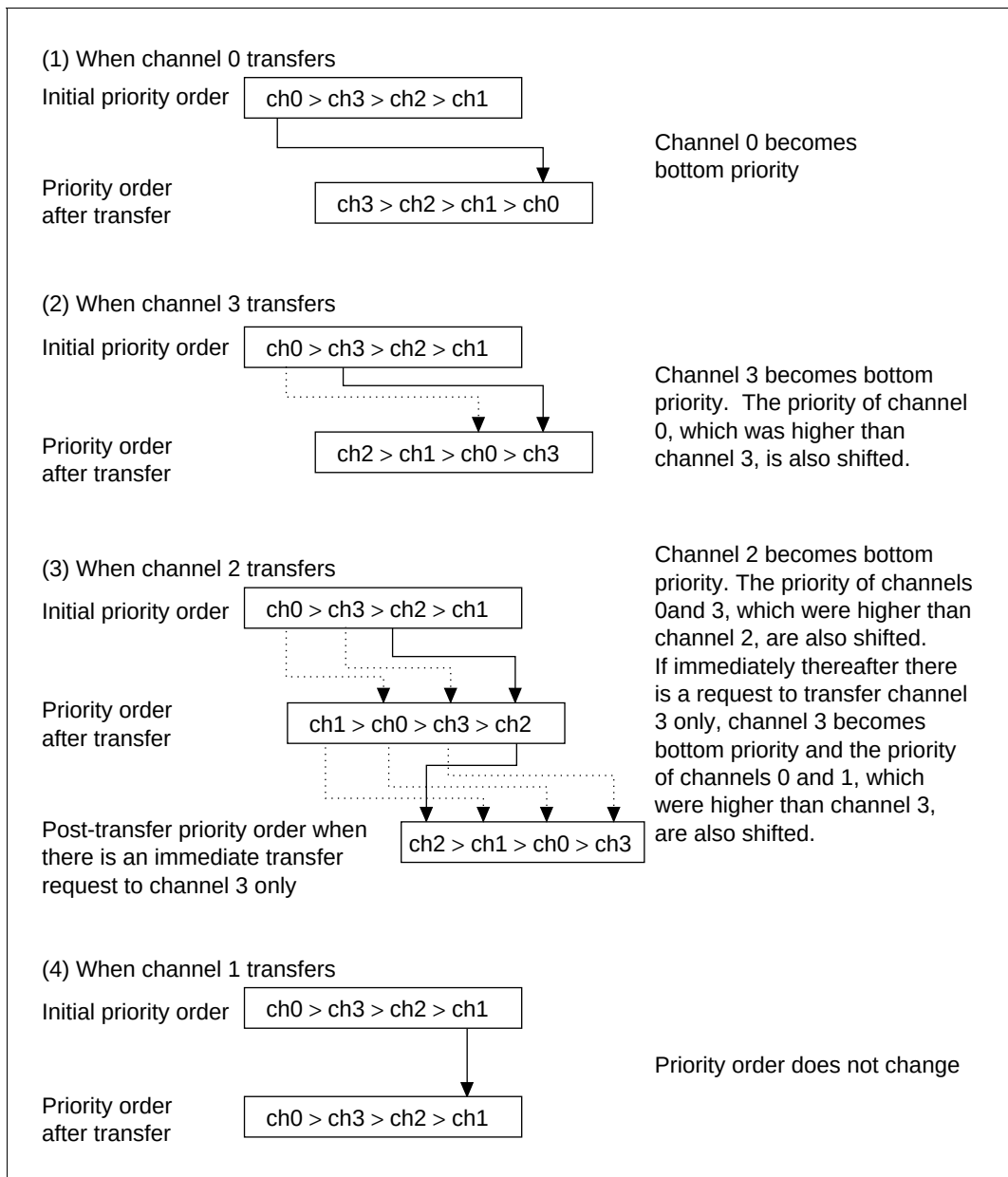
Figure 9.3 Round-Robin Mode
