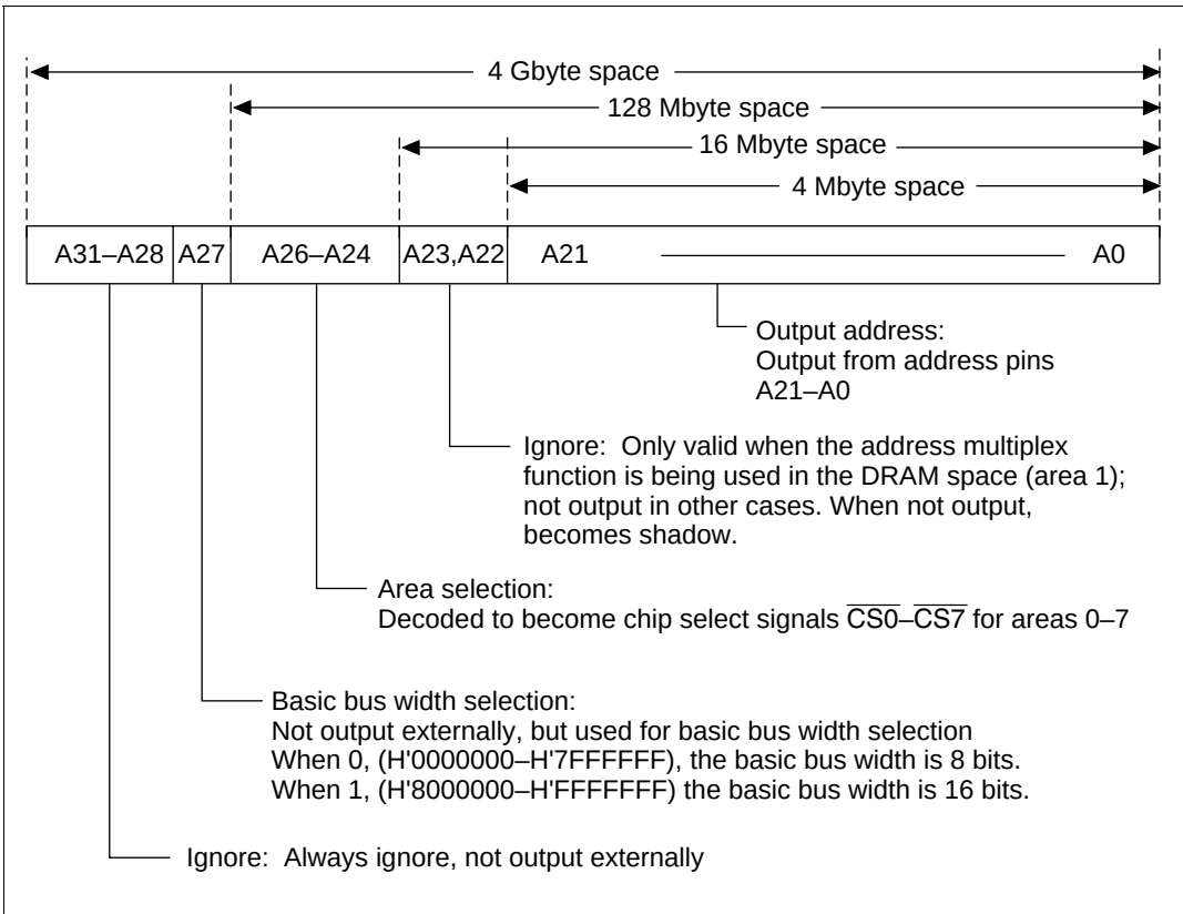
Figure 8.3 Address Format
