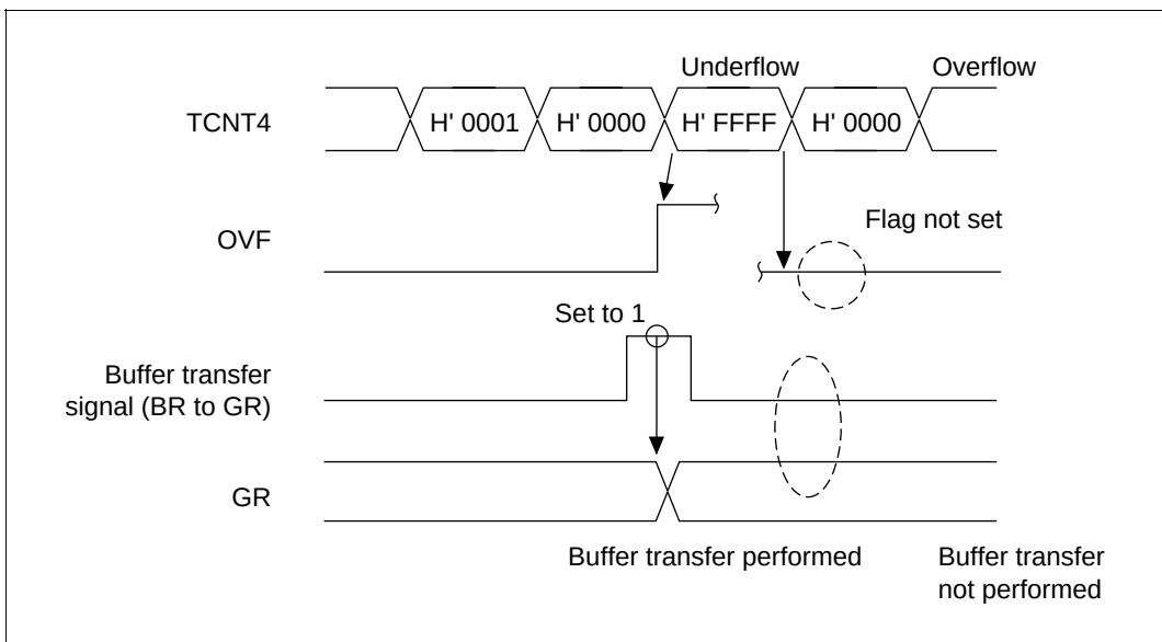
Figure 10.37 Undershoot Timing
