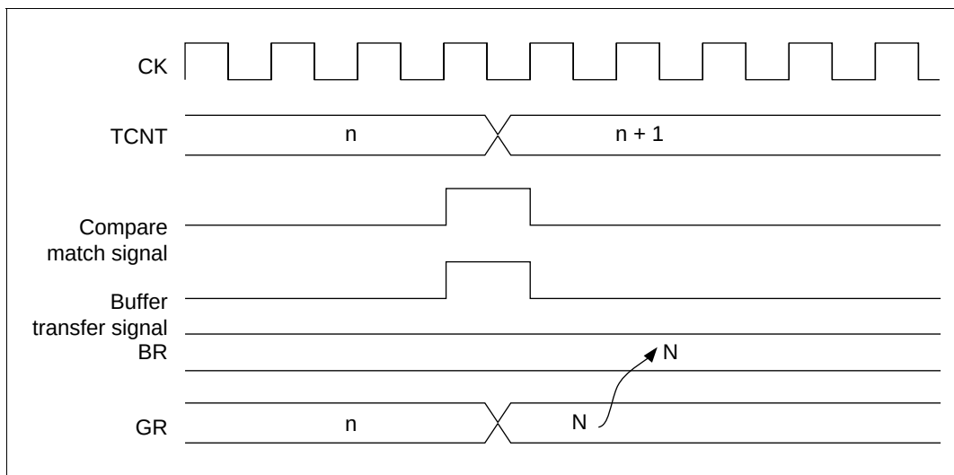
Figure 10.49 Compare Match Timing Example for Buffer Operation
