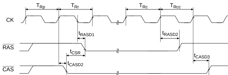
Figure 19.31 Self Refresh
