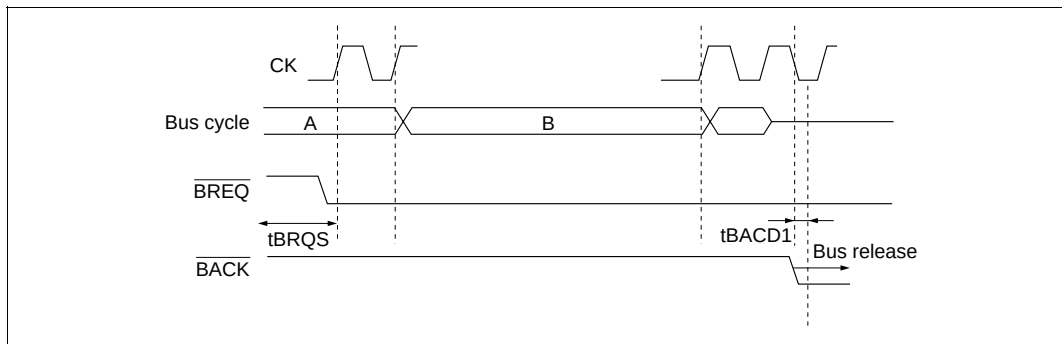
Figure 8.43 When \overline{\text{BREQ}} is Input without Satisfying \text{tBRQS}
