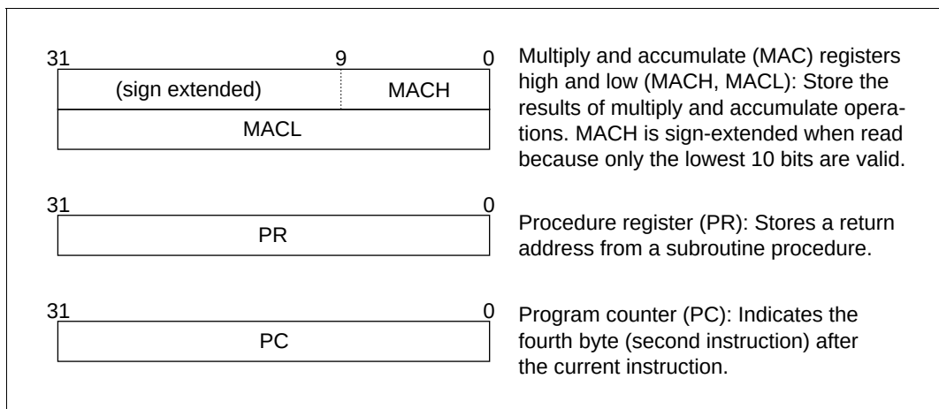
Figure 2.3 System Registers
