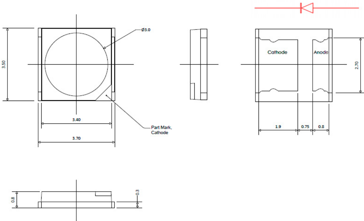
Figure 7b. Mechanical dimensions for L1SP-PRPxx03500000.
