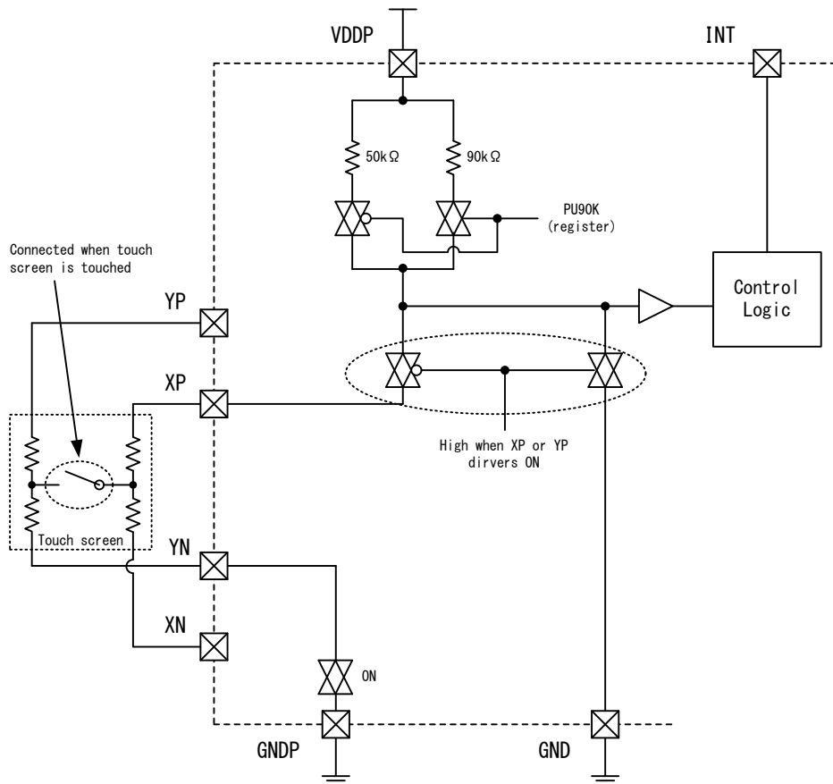
Figure 4. Touch detection circuit
