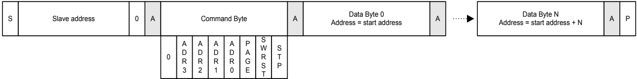
Figure 1. Write Protocol
