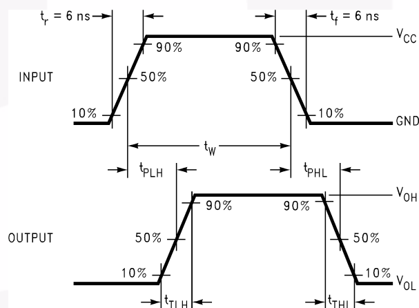
Figure 3. AC Waveforms
