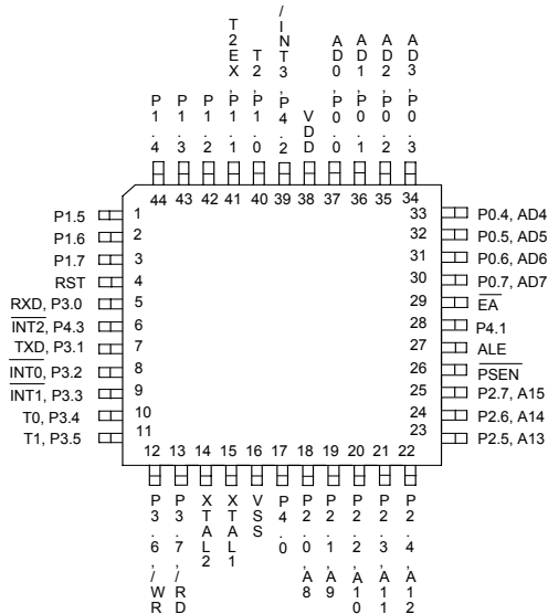
44-Pin QFP
