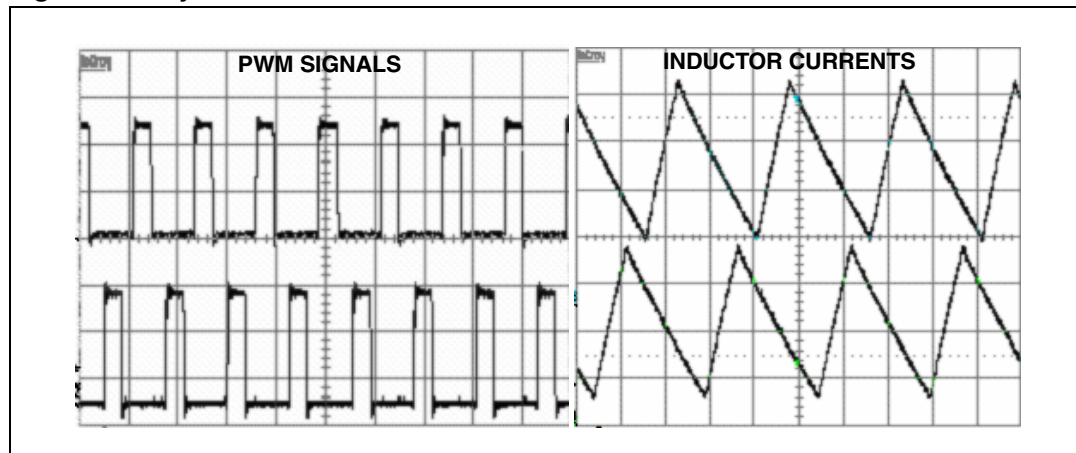
Figure 24. Synchronization
