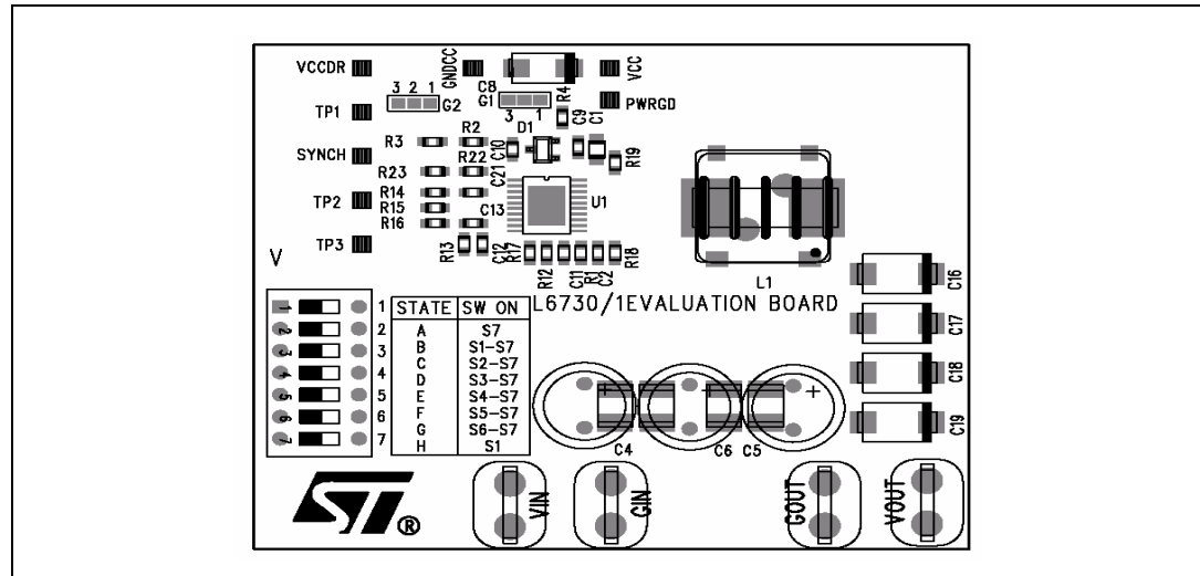
Figure 38. Demonstration board
