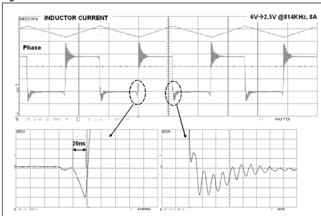
Figure 13. Dead times
