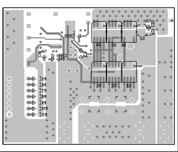
Figure 36. Bottom layer
