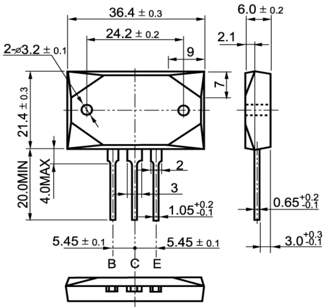
Fig.2 Outline dimensions
