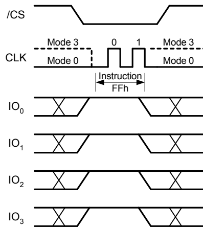
Figure 40. Disable QPI Instruction (QPI Mode only)
