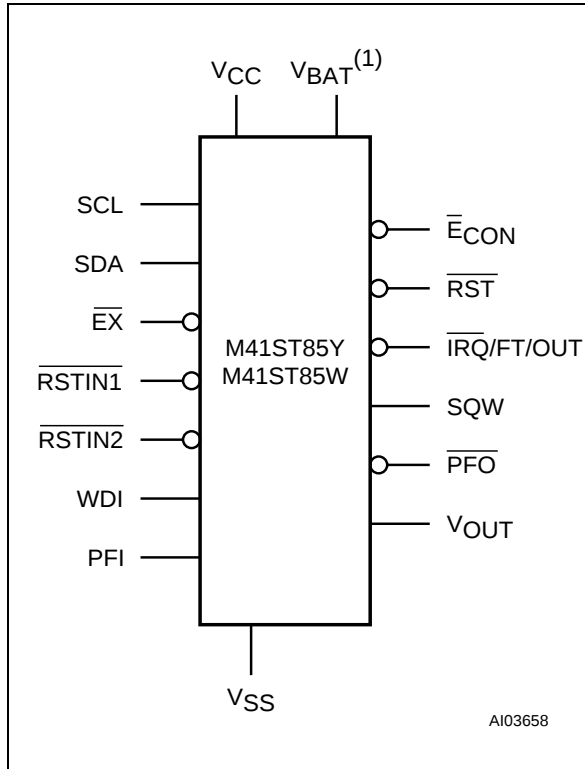
Figure 3. Logic Diagram
