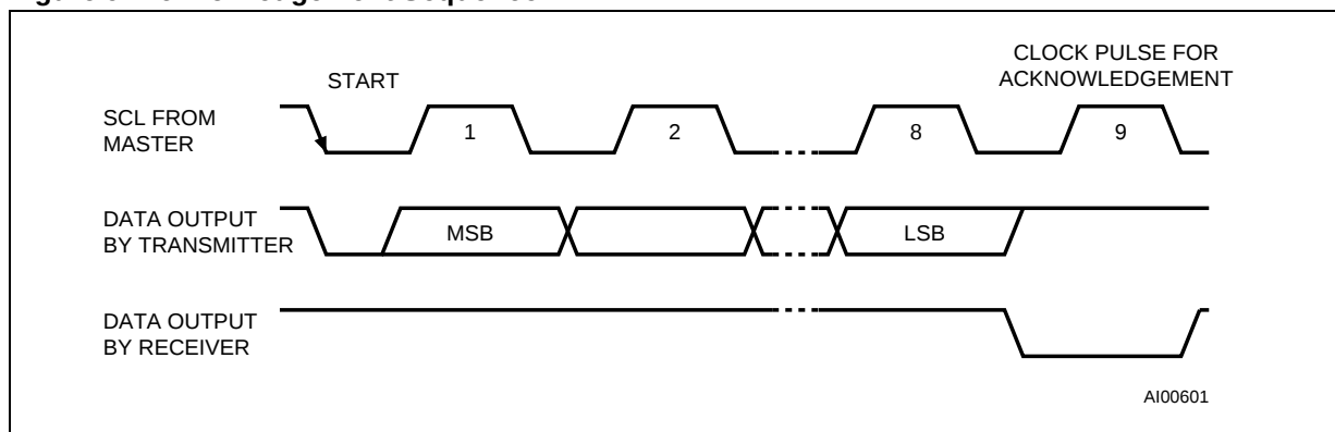
Figure 9. Acknowledgement Sequence
