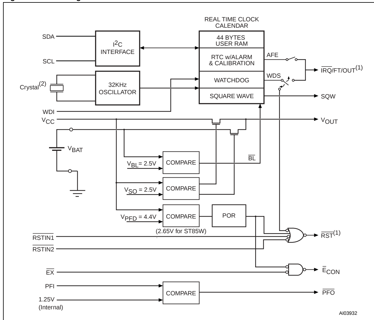
Figure 6. Block Diagram
