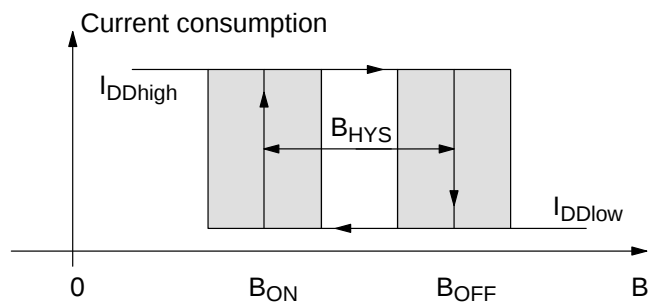
Fig. 4–5: Definition of magnetic switching points for the HAL581
