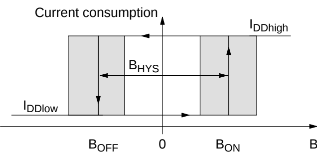
Fig. 1-3: Latching Sensor
