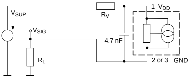
Fig. 5–2: Application Circuit 2
