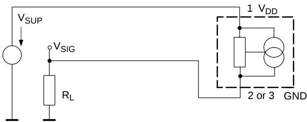
Fig. 5–1: Application Circuit 1
