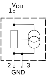
Fig. 1-4: Pin configuration
