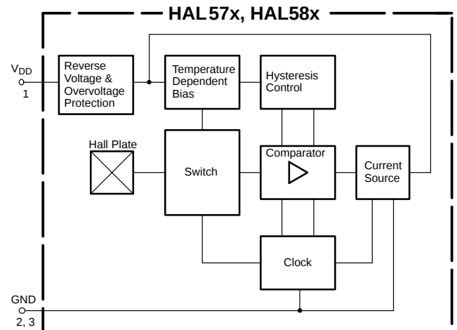
Fig. 2-1: HAL57x, HAL58x block diagram
