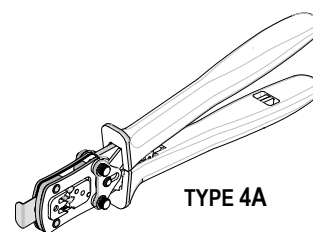
Hand Crimp Tool Order No. 63825-2100
