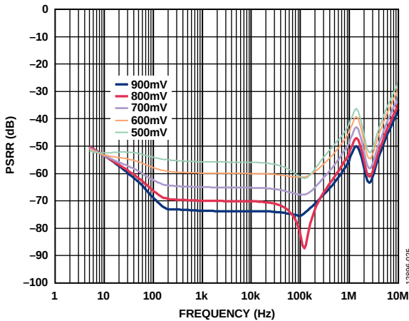
Figure 25. Power Supply Rejection Ratio (PSRR) vs. Frequency at Various Headroom Voltages, V_{OUT} = 1.8\text{ V} , 2 A Load
