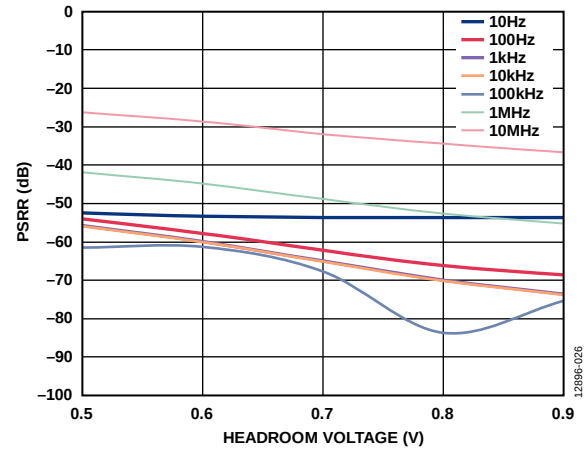
Figure 26. Power Supply Rejection Ratio (PSRR) vs. Headroom Voltage at Various Frequencies, V_{OUT} = 1.8\text{ V} , 2 A Load
