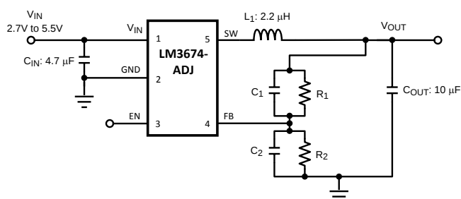
Typical Application Circuit for Adjustable Voltage Option
