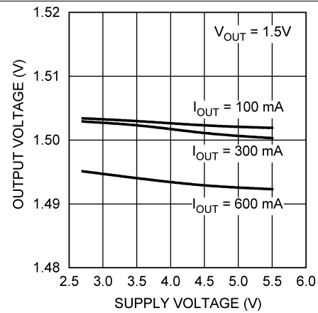
Figure 4. Output Voltage vs Supply Voltage
