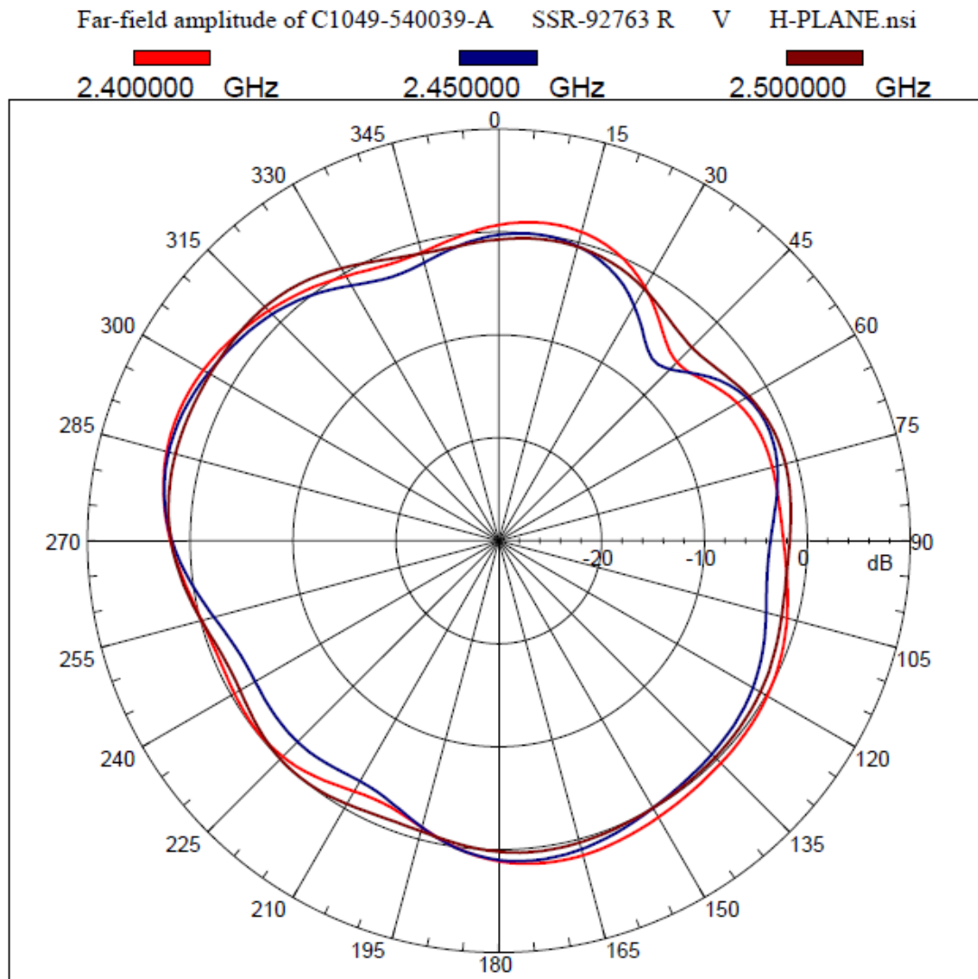
H-Plane Radiation Pattern of Right Antenna
