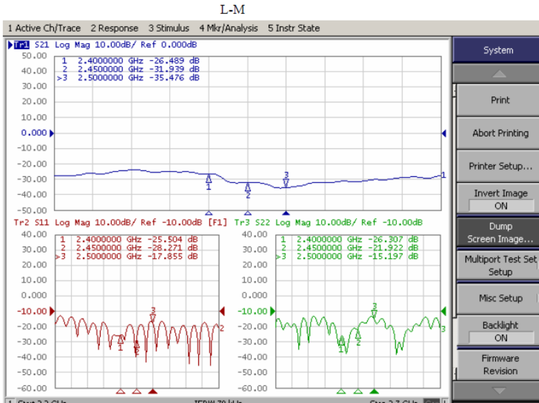
Return Loss and Isolation of Left and Middle Antenna
