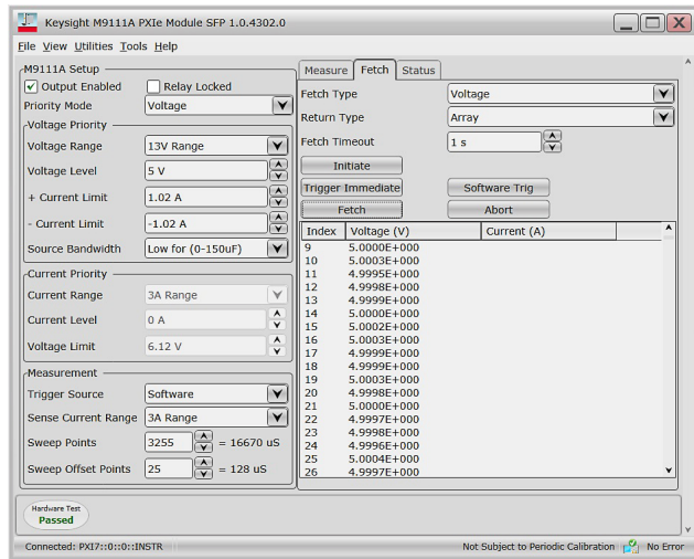
Figure 1. Soft front panel
