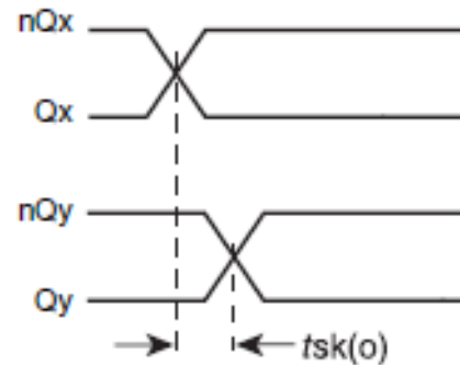
Figure 8. Output-to-Output Skew
