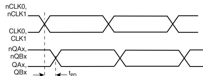
PROPAGATION DELAY
