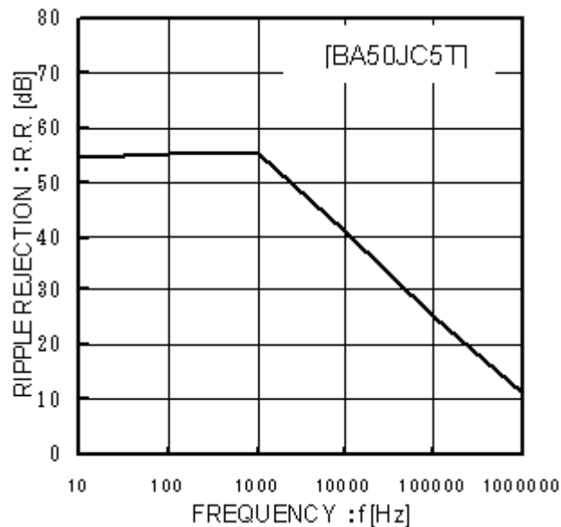
Fig.8 Ripple Rejection
