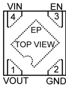
4-Pin 1mm × 1mm Thin DFN (MT)
