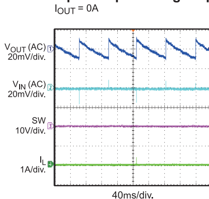
Input/Output Voltage Ripple
