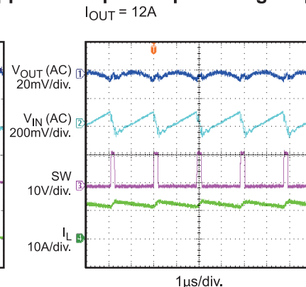
Input/Output Voltage Ripple
