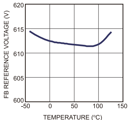
FB Reference Voltage vs. Temperature
