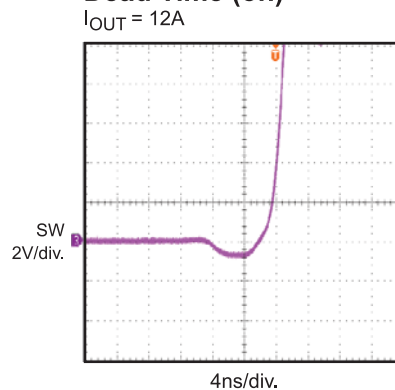
Dead Time (on)
