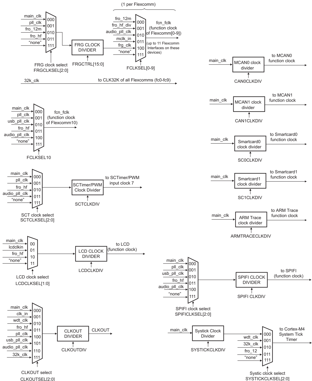
Fig 12. LPC540xx clock generation (continued)
