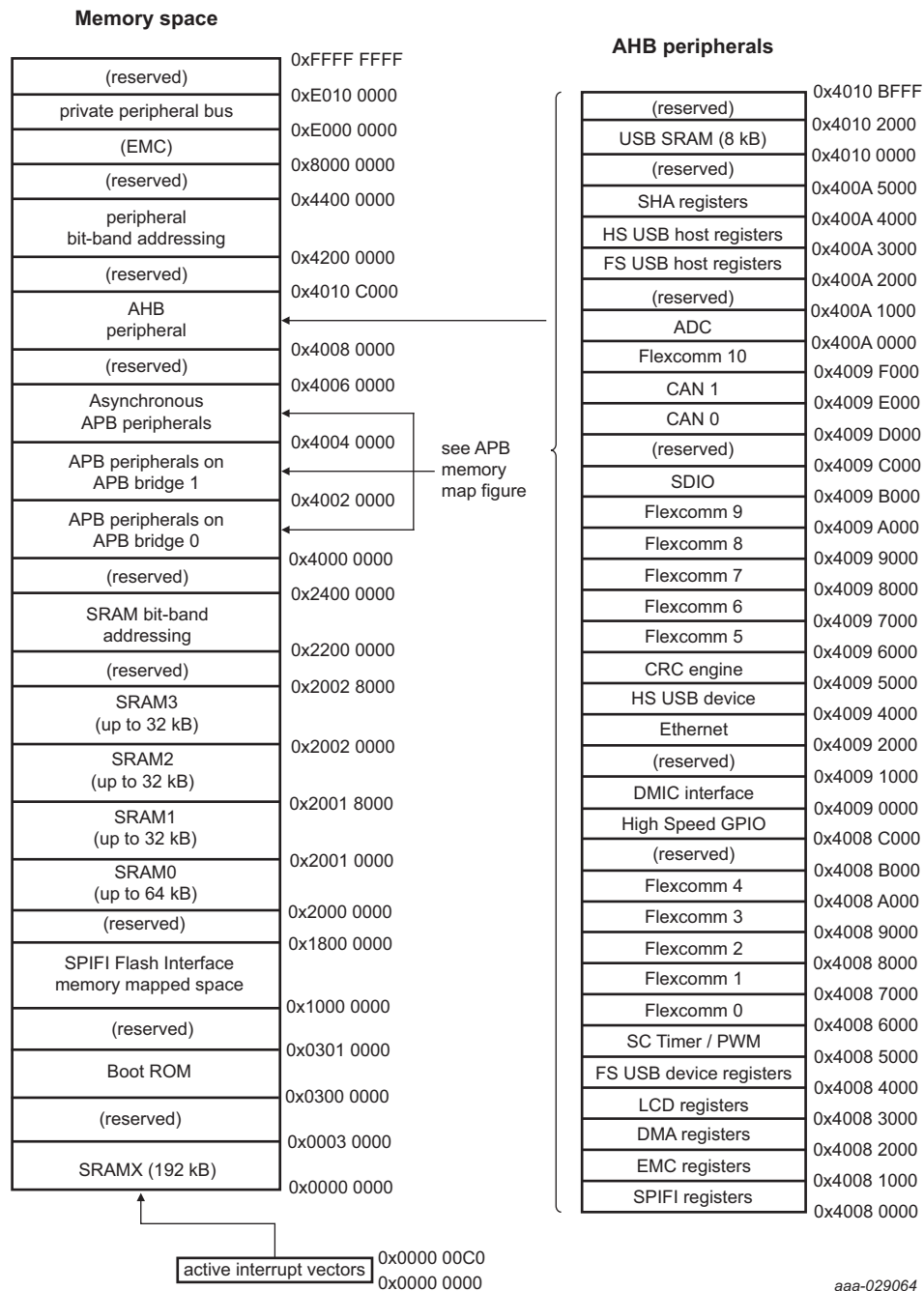
Fig 9. LPC540xx Memory mapping
