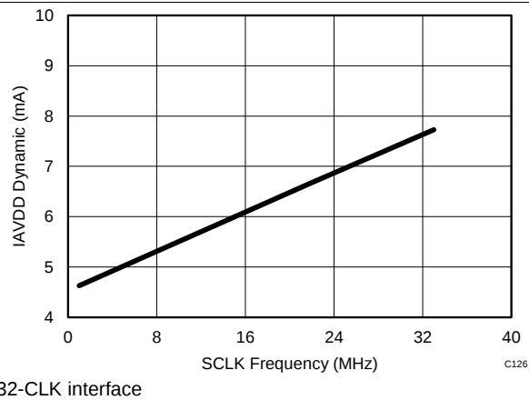
Figure 67. Analog Supply Current vs SCLK Frequency
