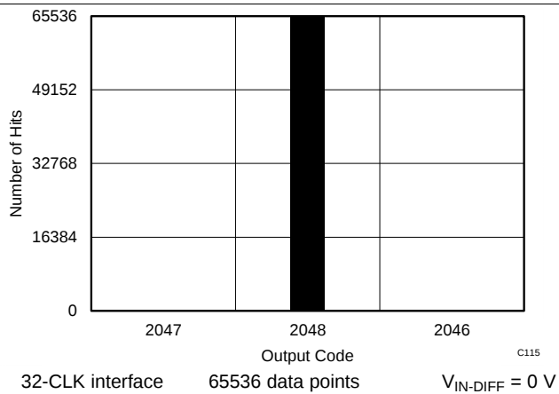
Figure 69. DC Histogram
