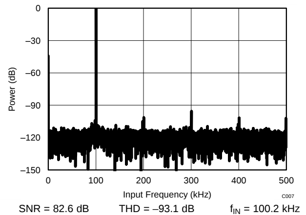
Figure 111. ADS7854 in 32-CLK Interface Mode
