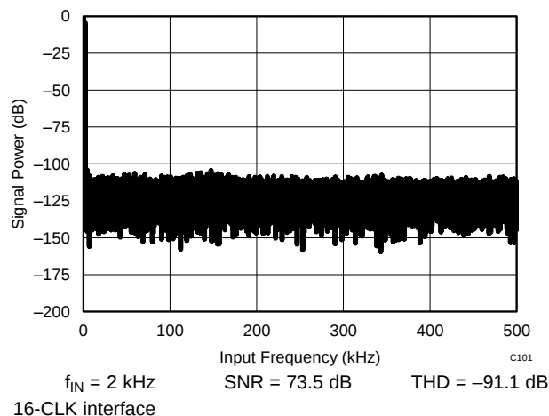
Figure 52. Typical FFT
