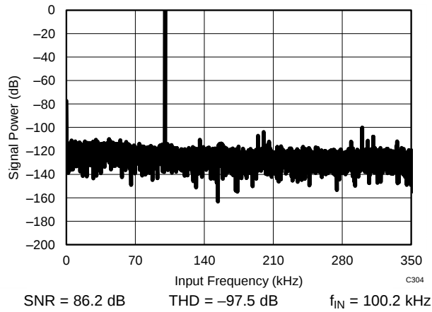
Figure 110. ADS8354 in 32-CLK Interface Mode
