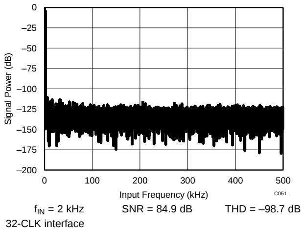
Figure 26. Typical FFT
