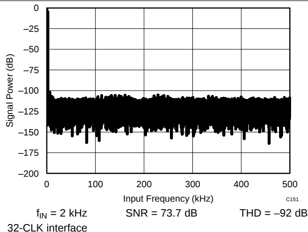
Figure 54. Typical FFT
