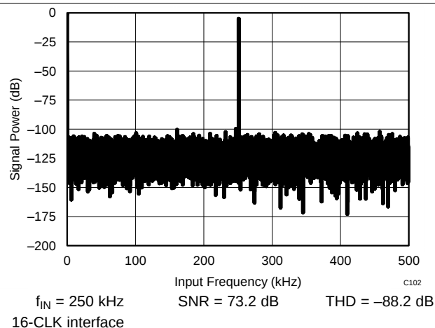
Figure 53. Typical FFT
