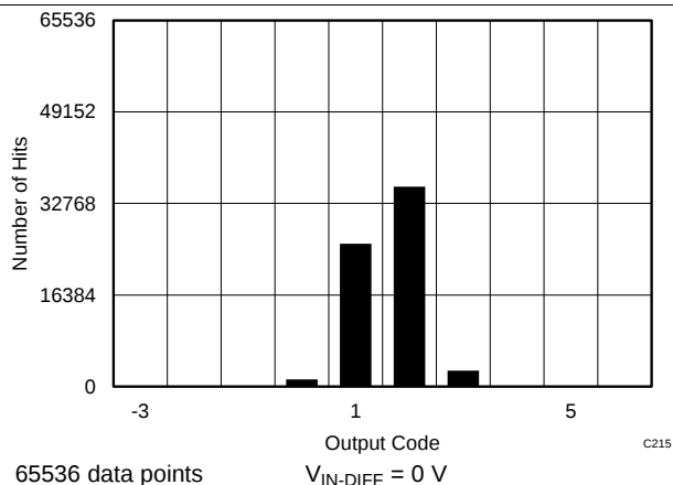
Figure 13. DC Histogram
