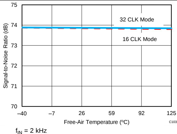
Figure 56. SNR vs Temperature
