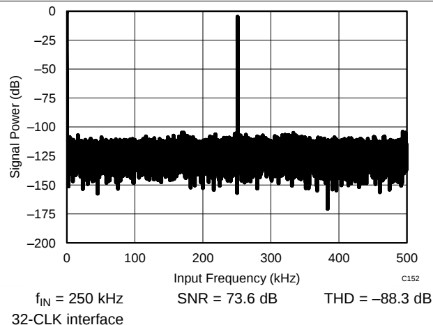
Figure 55. Typical FFT
