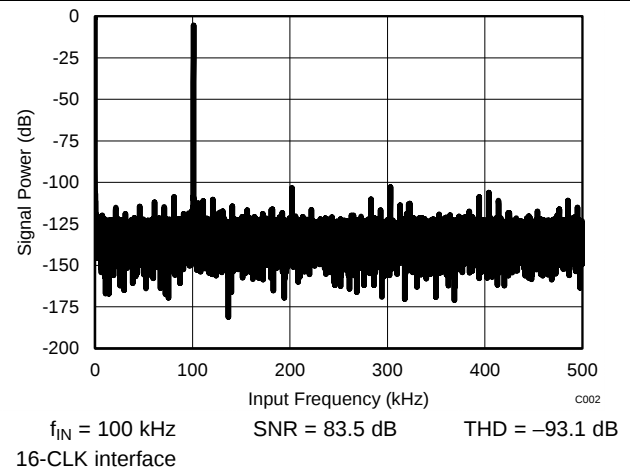
Figure 25. Typical FFT
