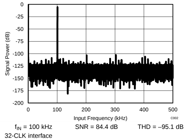
Figure 27. Typical FFT
