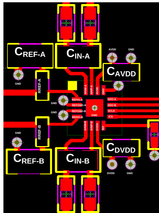
Figure 116. Recommended Layout
