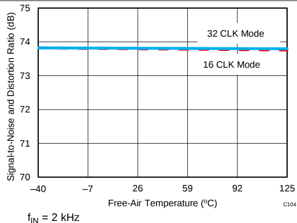
Figure 57. SINAD vs Temperature
