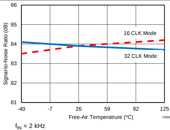
Figure 28. SNR vs Temperature
