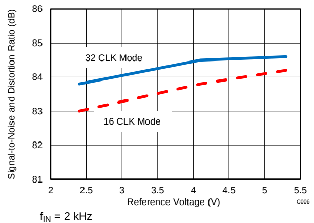
Figure 31. SINAD vs Reference Voltage
