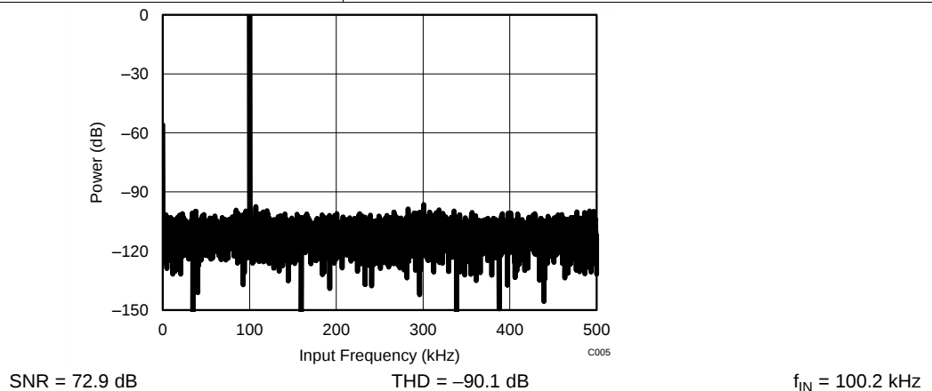
Figure 112. ADS7254 in 32-CLK Interface Mode
