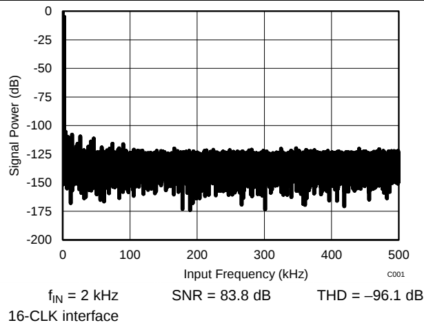
Figure 24. Typical FFT
