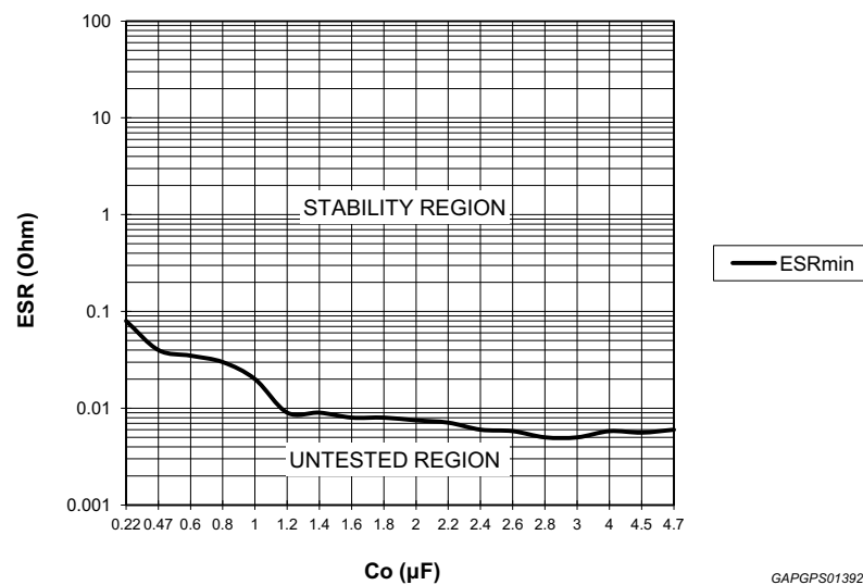
Figure 15. Stability region
