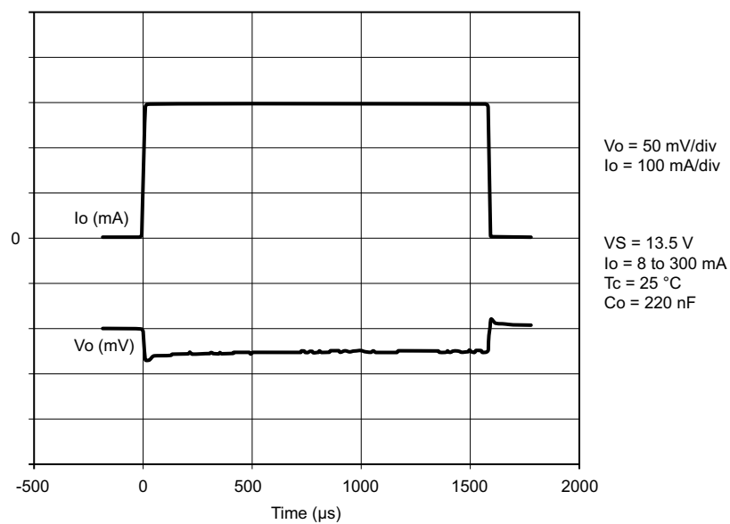
Figure 16. Maximum load variation response
